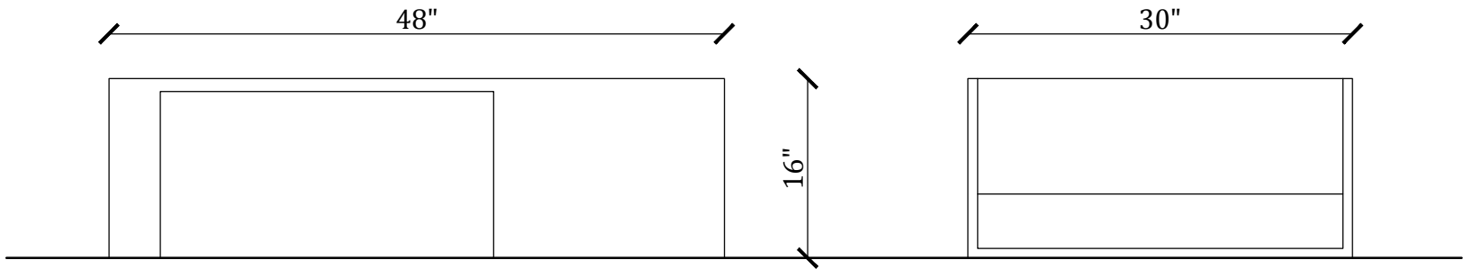
SIDE VIEW
